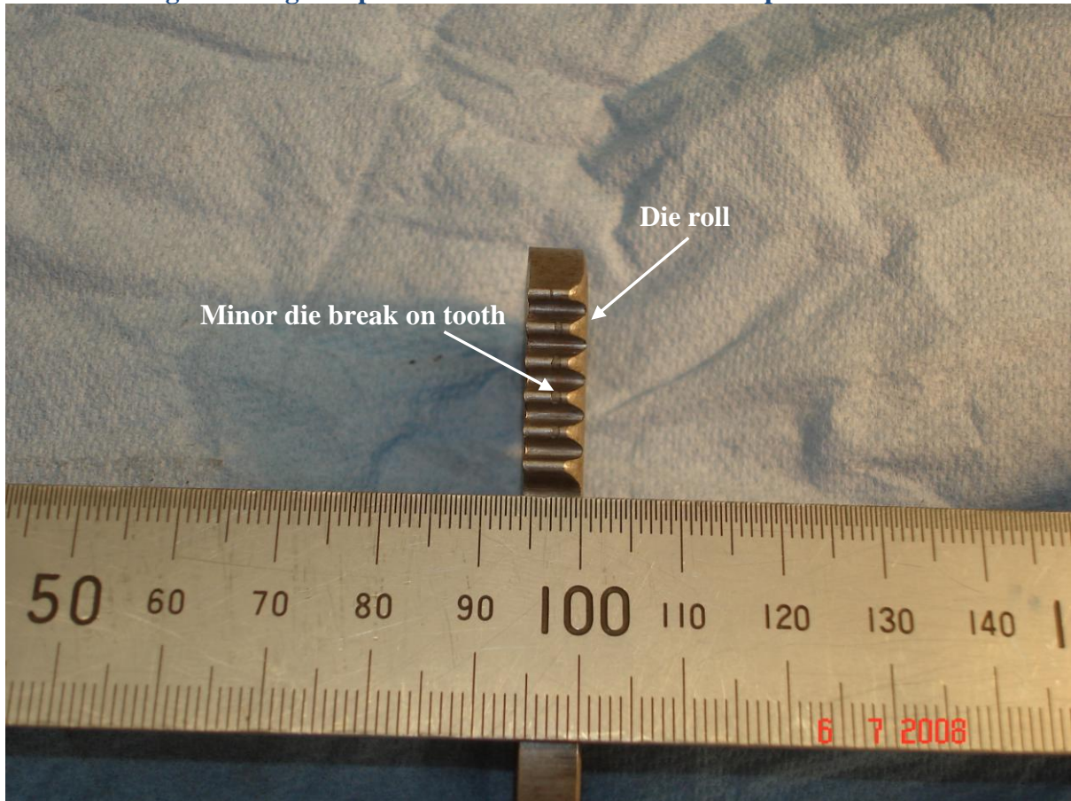
Image depicting component produced from next generation DC Ross fine blank tooling
